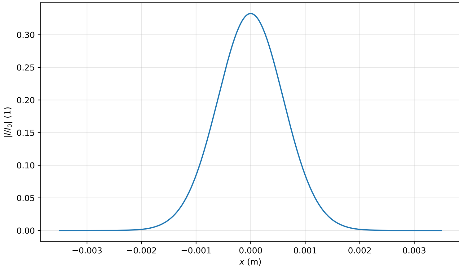
Intensity profile I(x, y = 0, z = 3.025m)/I_0 , P_{in}=0.1P_{cr} , artificial time
